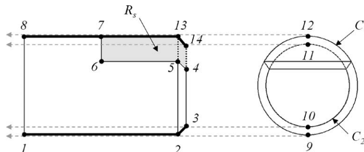
Fig. 11. Rotational profile generation through symmetry test.
