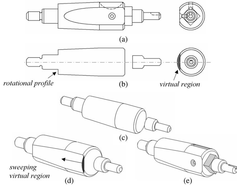
Fig. 15. Shaft drawing.
