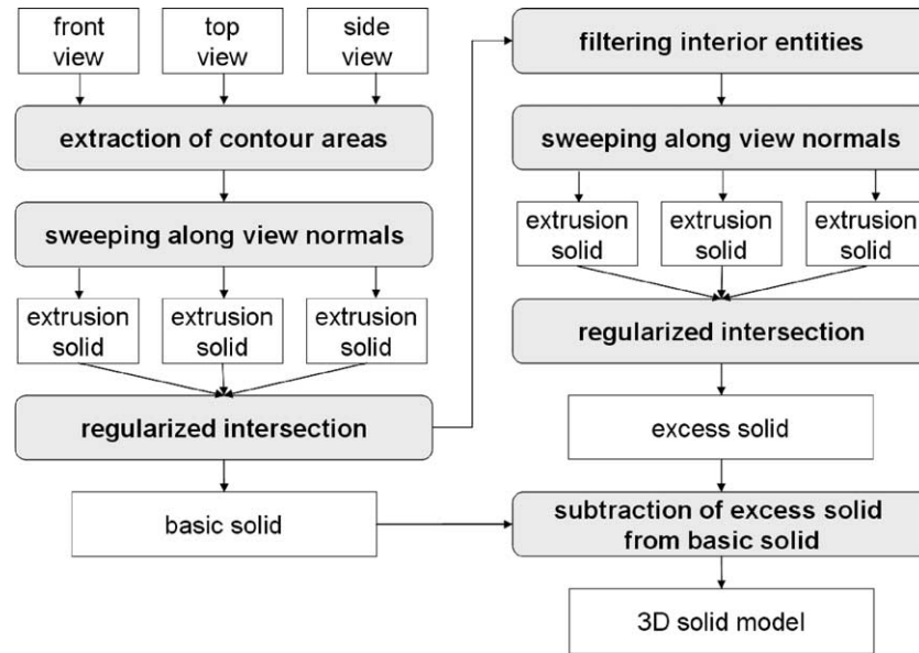
Fig. 2. Two-stage extrusion algorithm [14].
