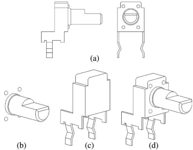
Fig. 14. Switch drawing.
