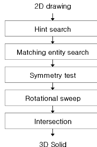
Fig. 6. Hint-based solid reconstruction process.
