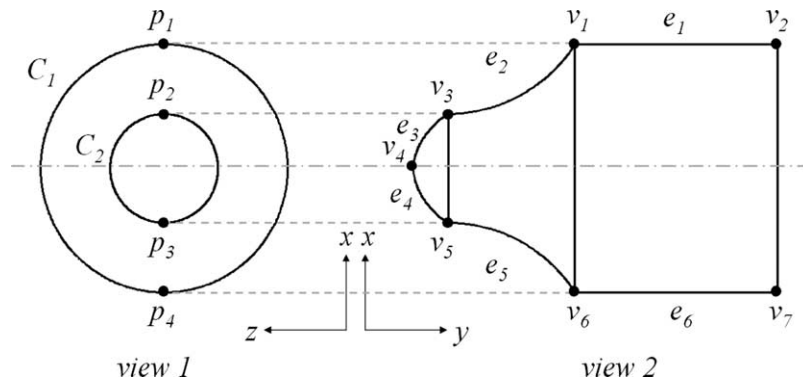
Fig. 4. Matching vertices and matching edges.
