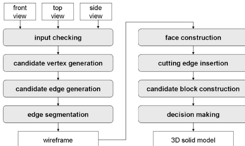
Fig. 1. A typical pipeline of B-rep based approach.
