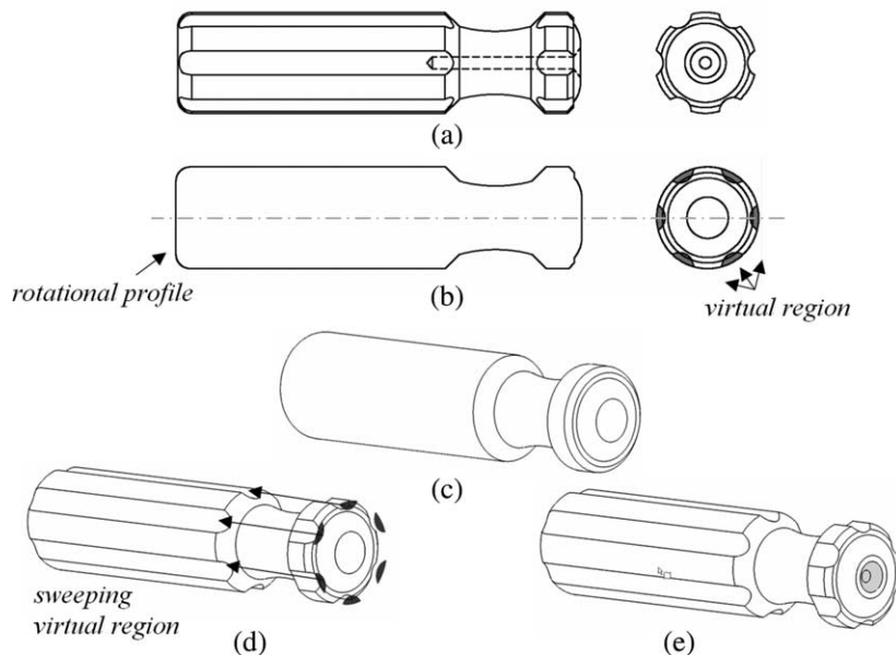
Fig. 16. Screwdriver drawing.
